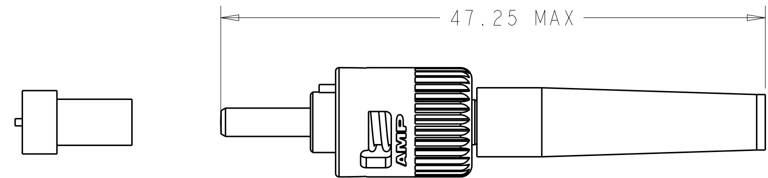
ASSEMBLED CONNECTOR (SHORT BOOT)
