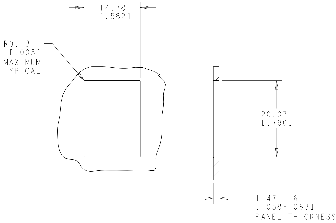
SINGLE PANEL CUTOUT
