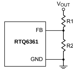
Figure 6. Output Voltage Setting
