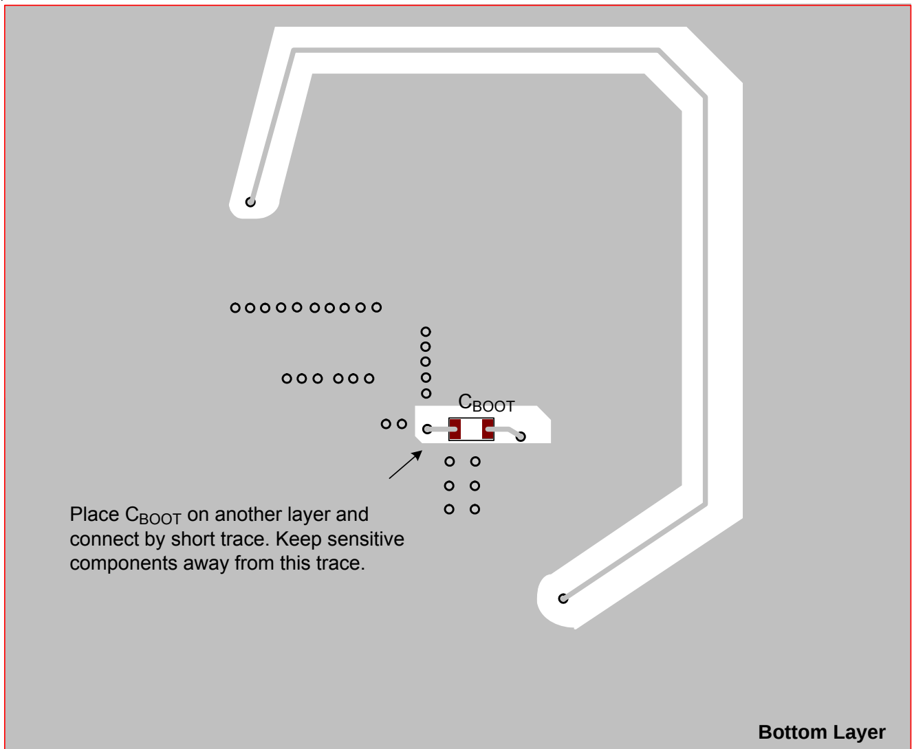
Figure 17. Layout Guide for RTQ6361GQW (Bottom Layer)
