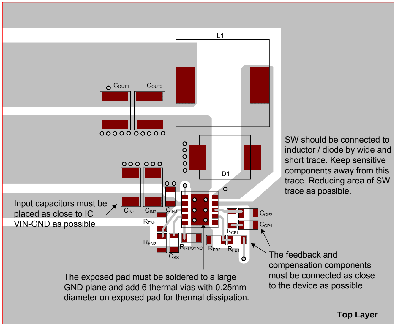
Figure 16. Layout Guide for RTQ6361GQW (Top Layer)
