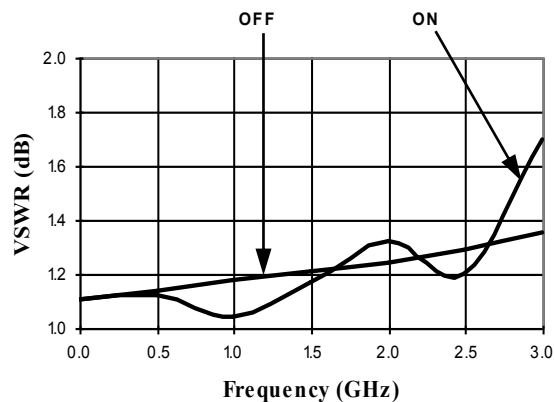
Typical VSWR
