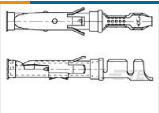
TE Part #163088-1 062 SOC.ASS. TYP3+
