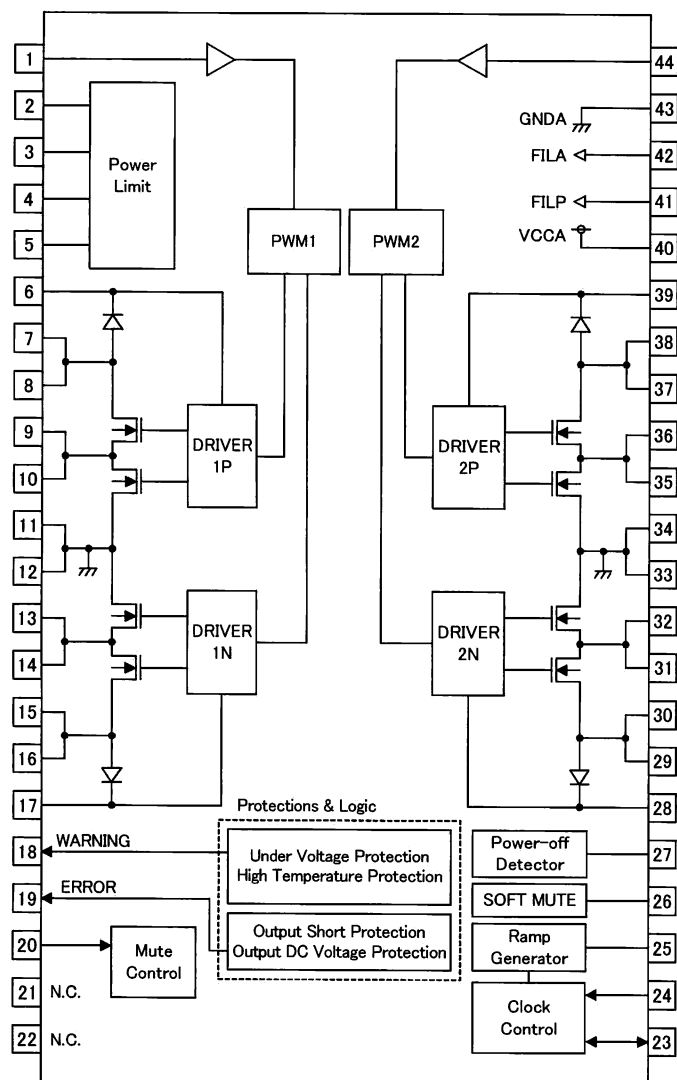
Block diagram
