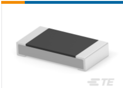
TE Part #3-2176392-6 RQ 1206 309K 0.1% 10PPM 5K RL
