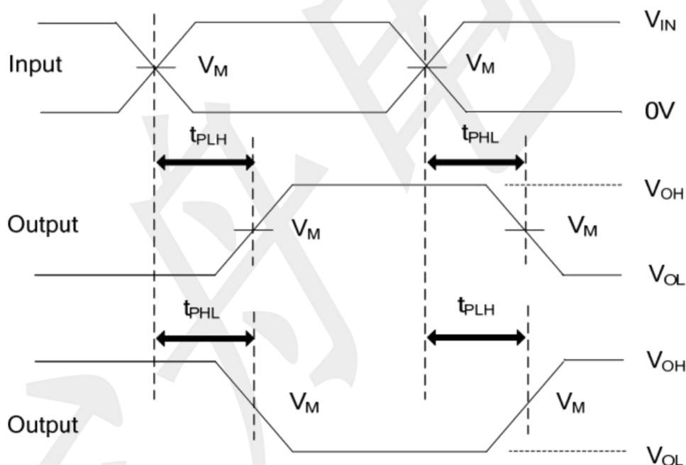
PROPAGATION DELAY TIMES
