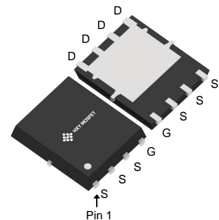
DFN5X6-8L DFN-8(5.1x5.7))
