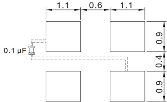
Footprint (Recommender)
