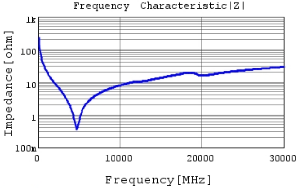
GRM0225C1H7R0WA03 |Z| DCOV, 25degC
