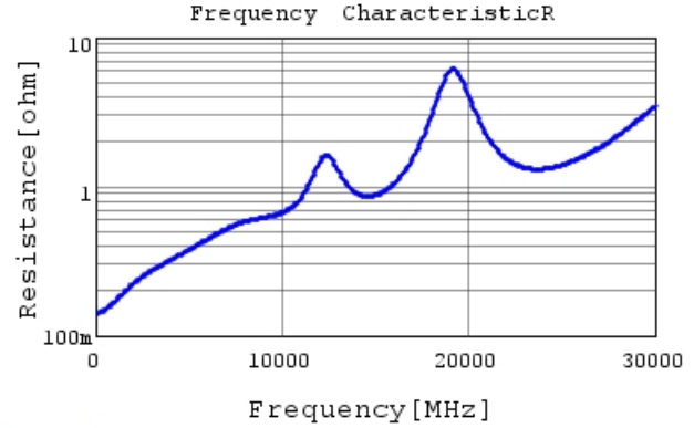
GRM0225C1H7R0WA03 R DCOV, 25degC
