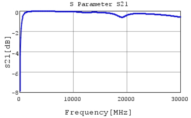
GRM0225C1H7R0WA03 S21 DCOV, 25degC
