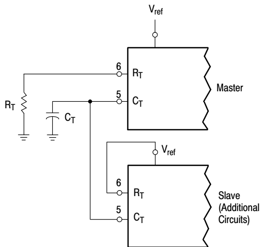
Figure 19. Slaving Two or More Control Circuits
