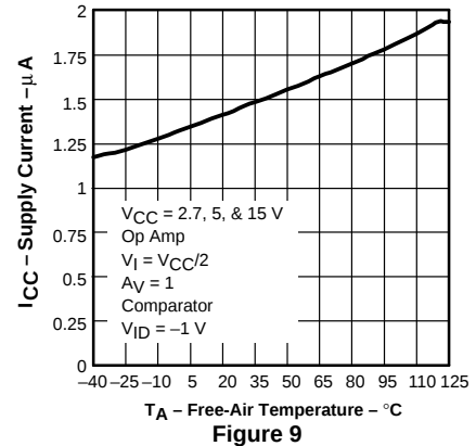
SUPPLY CURRENT vs FREE-AIR TEMPERATURE
