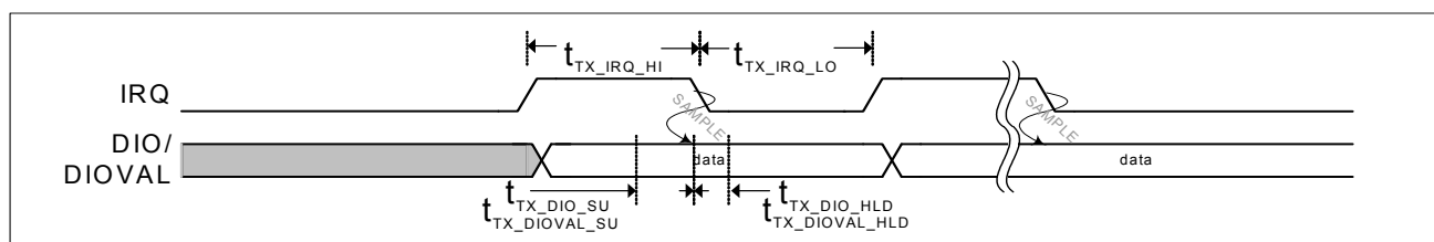
Figure 14. DIO Transmit Timing Diagram
