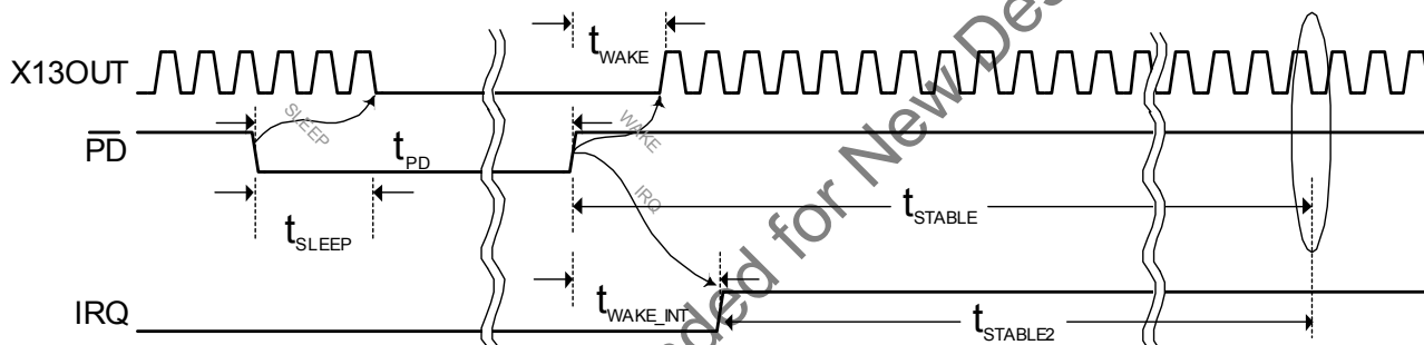
Figure 16. Sleep / Wake Timing
