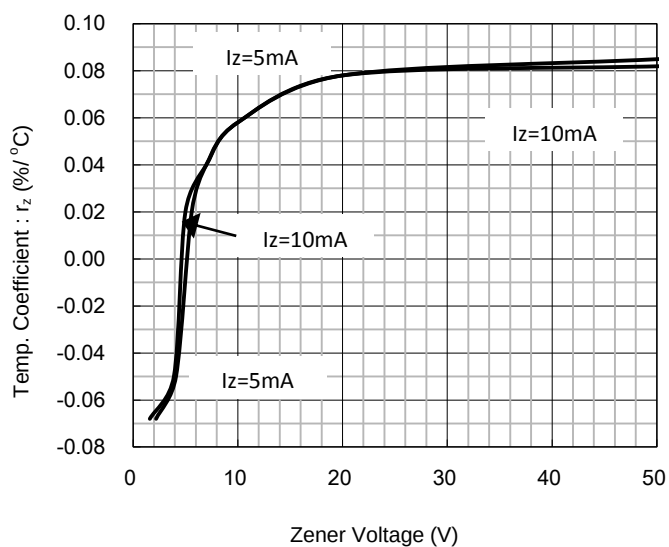
Fig.2 r_z - V_Z Characteristics
