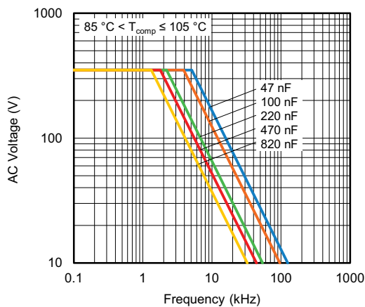
Maximum RMS voltage as a function of frequency (1000 V DC )
