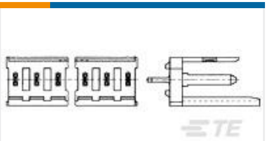
TE Part #280610-1 4P MOD 1 SHROUDED HEADER, ST, TIN PLTD
