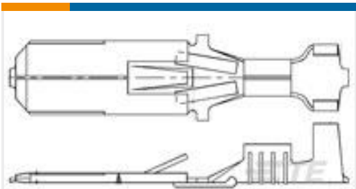
TE Part #42241-2 FF 250 TAB 18-14 AWG .032 TPBR
