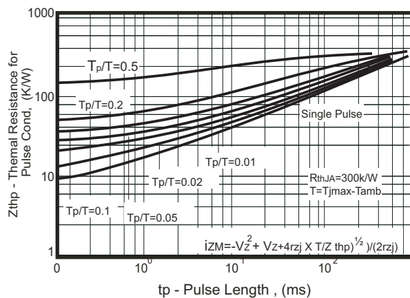
Fig.10- Thermal Response
