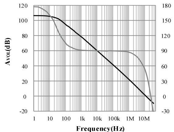
Fig. 5 Open-loop Gain and Phase as a function of Frequency
