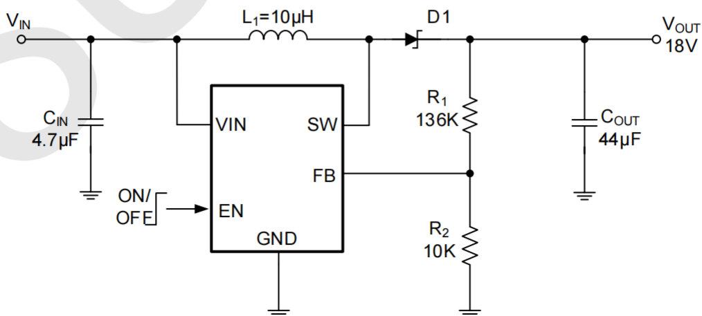
Boost Application Circuit
