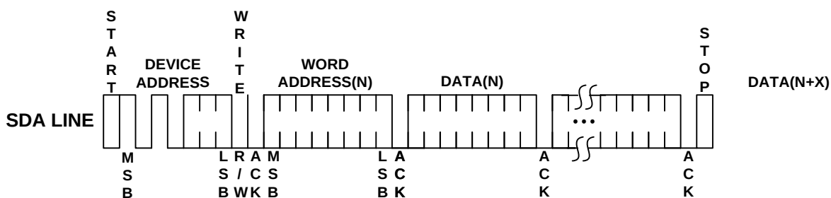
Figure 6: Page Write
