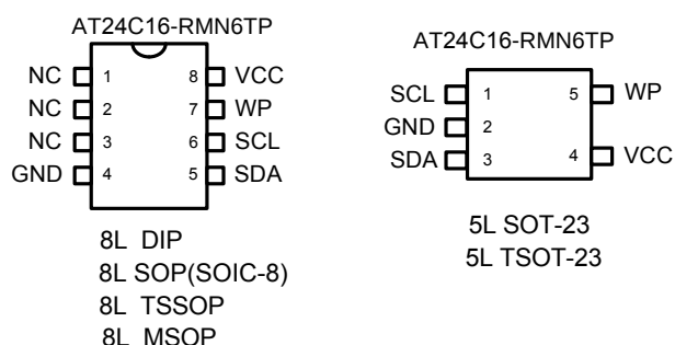
Figure 1: Package types
