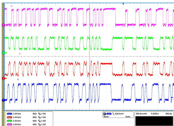
Figure 8-9. THVD2410V Waveforms at V_{CC} = 3.3 \text{ V}
