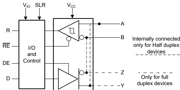
Figure 7-1. THVD2410 and THVD2450 Block Diagram
