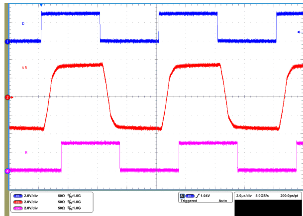
Figure 8-8. THVD2410V Waveforms at V_{CC} = 5 \text{ V}
