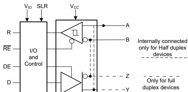
Simplified Schematic
