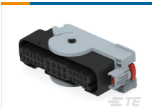
TE Part #7-2109446-2 MCP 1.5/2.8 SLD 30P PLUG ASSY
