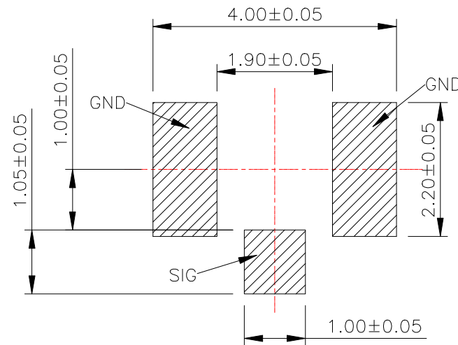
RECOMMENDED PCB LAYOUT 1 (GENERAL TOLERANCE IS \pm 0.05 )
