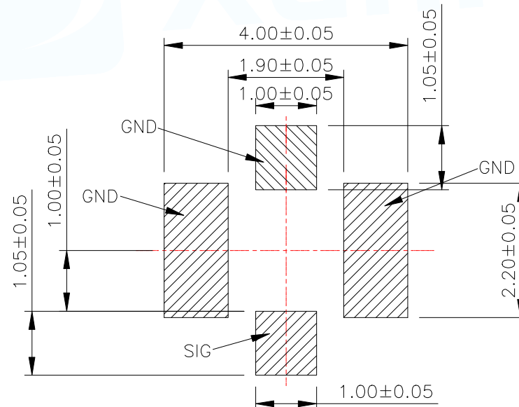
RECOMMENDED PCB LAYOUT 2 (GENERAL TOLERANCE IS \pm 0.05 )
