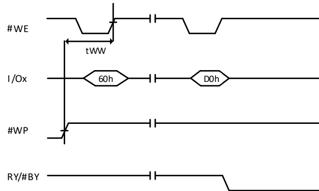
Figure 9-23 Erase Enable
