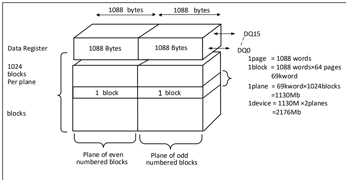
Figure 6-2 Array Organization
