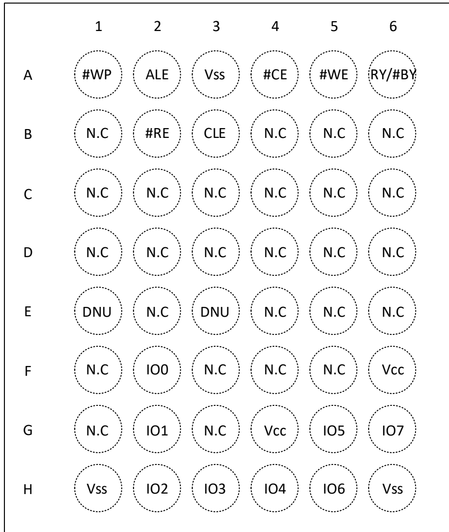
Figure 3-1 Ball Assignment 48-ball VFBGA (Package code D)
