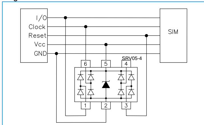
Figure 6 - SIM Port
