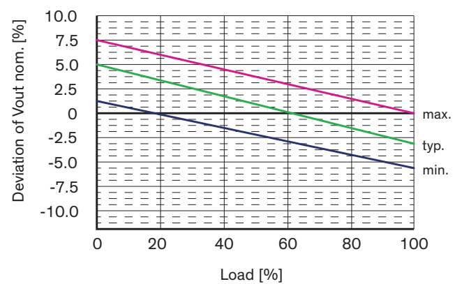
5 Vout models
