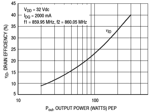
Figure 5. Two-Tone Drain Efficiency versus Output Power
