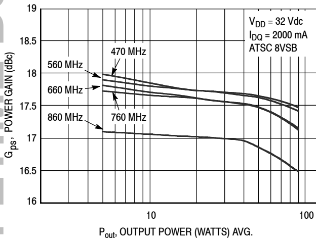
Figure 15. Single-Channel ATSC 8VSB Broadband Performance Power Gain versus Output Power
