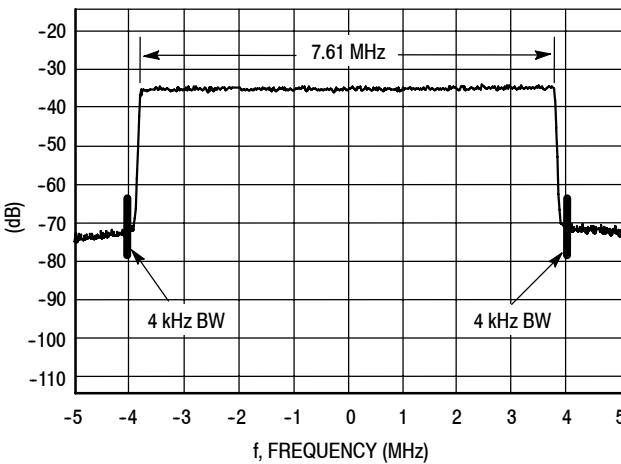
Figure 13. 8K Mode DVBT OFDM Spectrum
