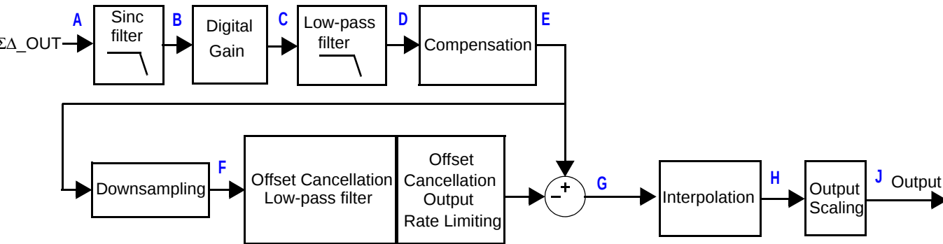
Figure 15. Signal-chain diagram
