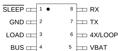
Figure 3. 33390 Pin Connections
