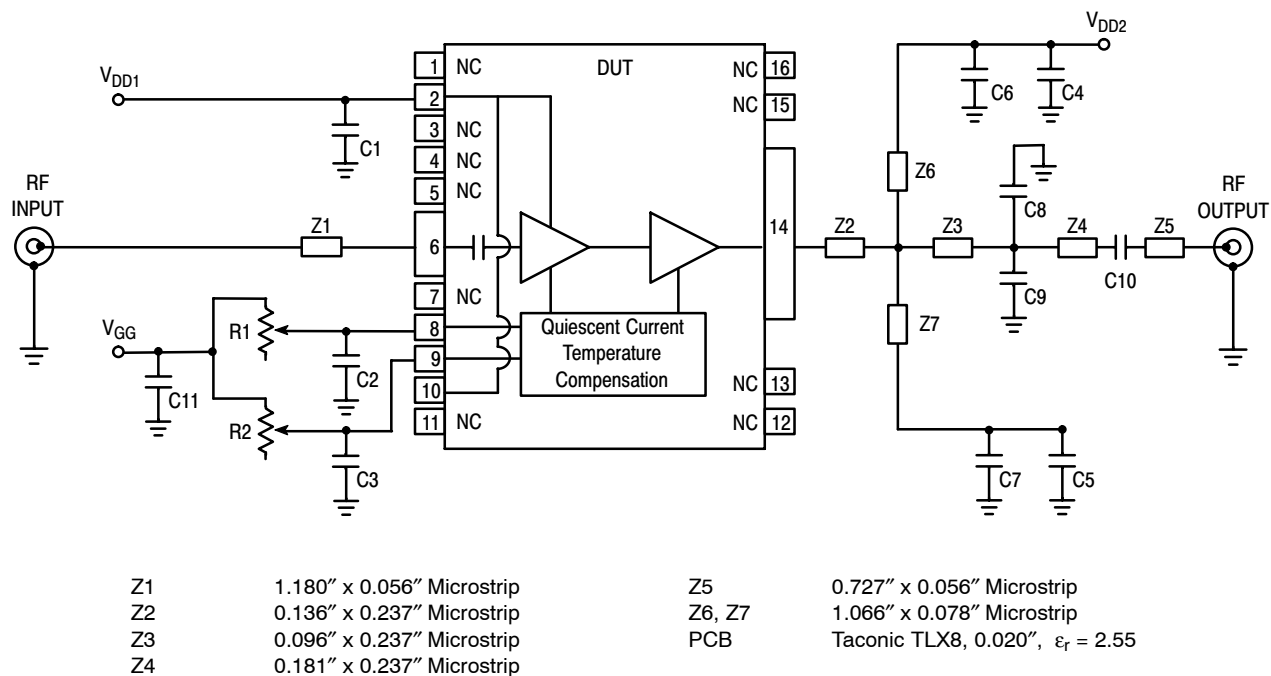
Figure 17. MW6IC2240NBR1(GNBR1) Test Circuit Schematic — TD-SCDMA
