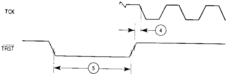
Figure 6-9. TRST Timing Diagram
