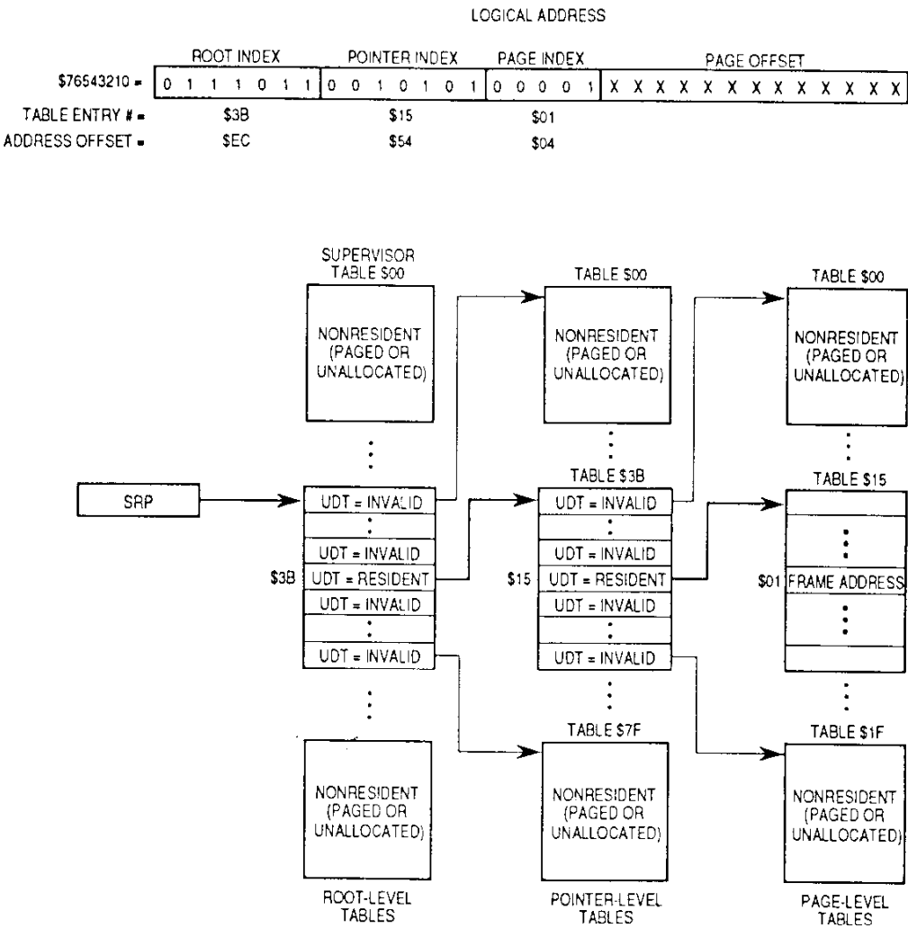
Figure 3-16. Translation Table with Nonresident Tables
