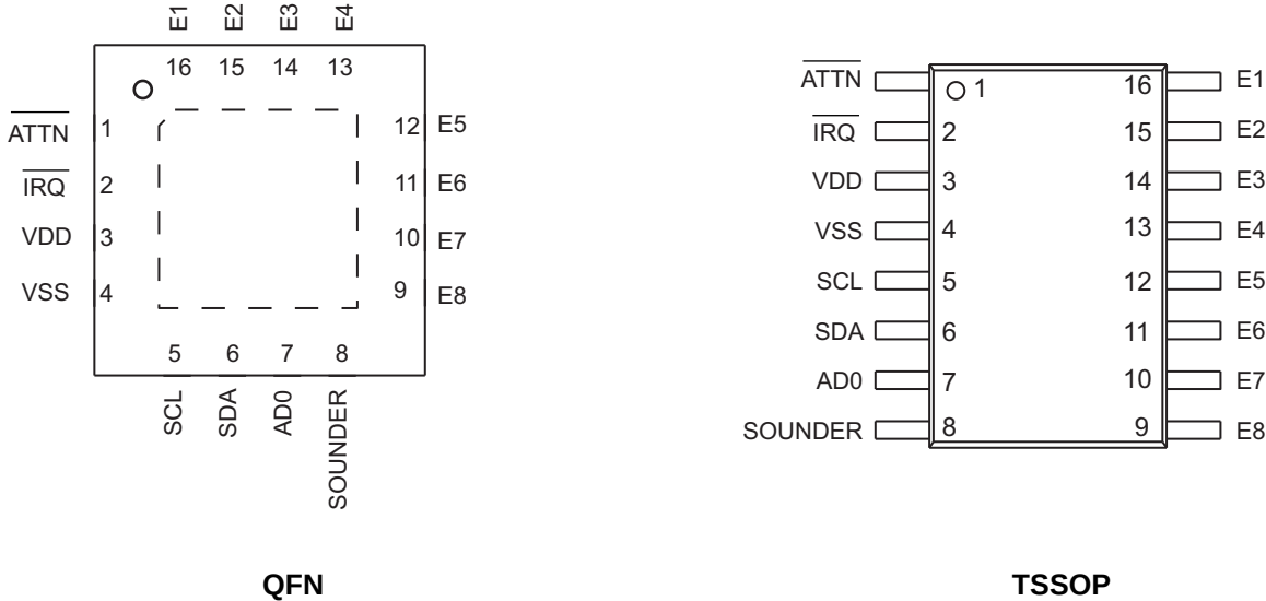
Figure 3. Package Pinouts
