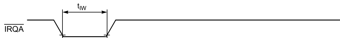
Figure 4-13 Recovery from Stop State Using Asynchronous Interrupt Timing
