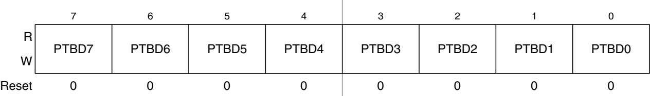
Figure 6-9. Port B Data Register (PTBD)
