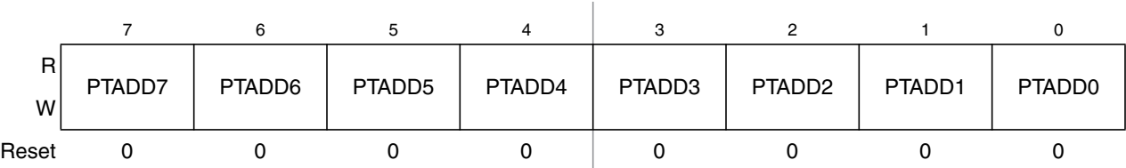
Figure 6-8. Data Direction for Port A (PTADD)
