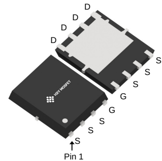
DFN5X6-8L (PQFN-8(4.9x5.8))
