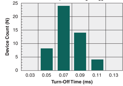
Typical Turn-Off Time (N=50, I_F=10\text{mA} , I_L=1A_{DC} )
