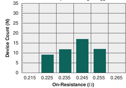
Typical On-Resistance Distribution (N=50, I_F=10\text{mA} , I_L=1A_{DC} )
