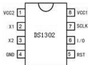
SOP-8(SOIC-8)
