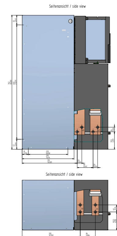
Dimensional Drawing 280
