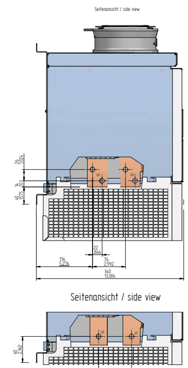
Dimensional Drawing 278
