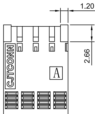
2x2P~2x7P
