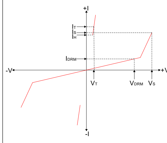
V-I Curve
