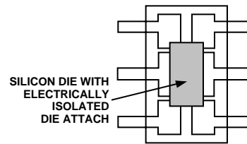
b. Thermally Enhanced Chip-on-Lead Package Figure 22.
