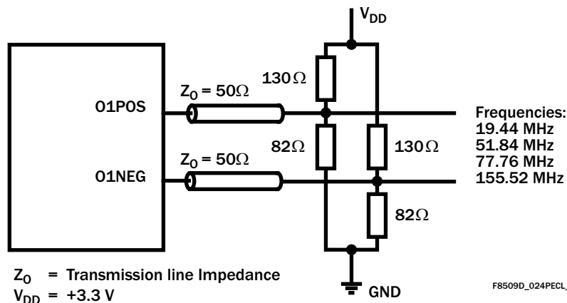
Figure 11 Recommended Line Termination for PECL Output Port
