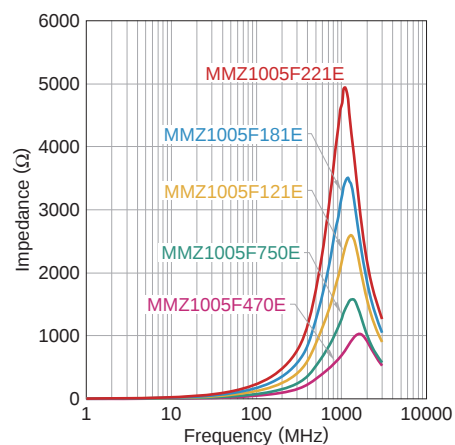
MMZ1005F-E series
