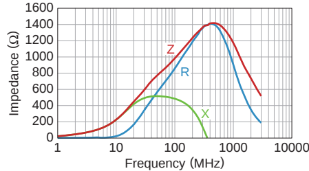
MMZ1005A102ET000
