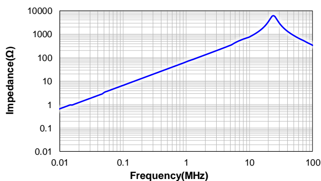
CPEX2626S-150MC
