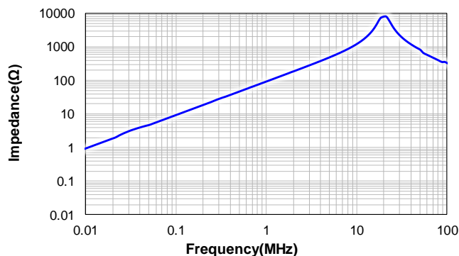
CPEX2626S-220MC
