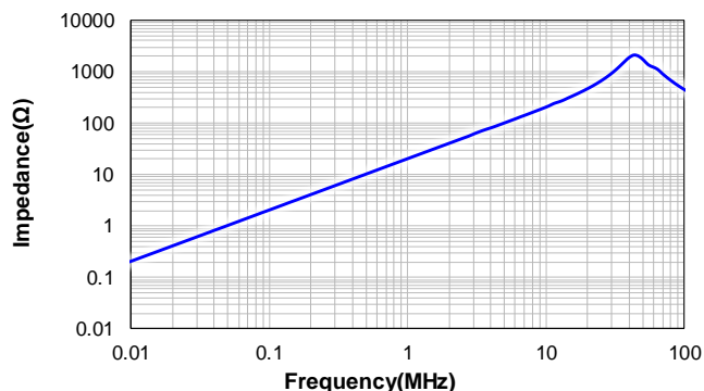
CPEX2626S-7R2MC
