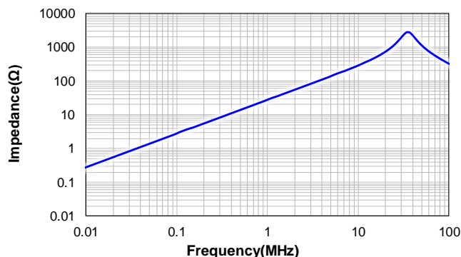
CPEX2626S-100MC
