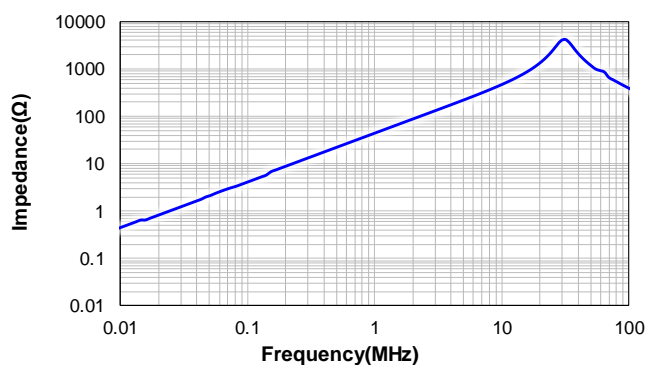
CPEX2626S-130MC
