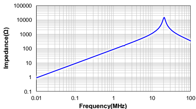
CPEX2626S-180MC
