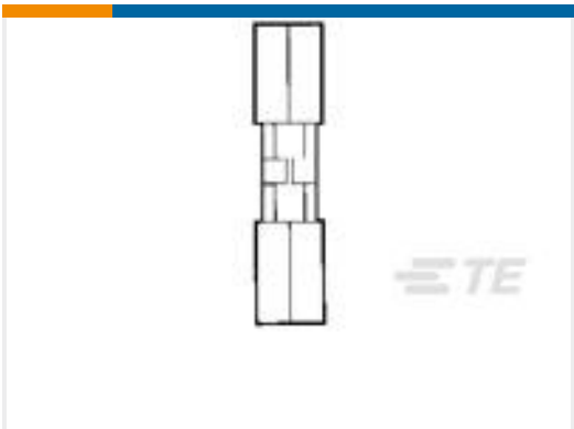
TE Part #321024 SPLICE, BUTT, BUDGET, 26-22
