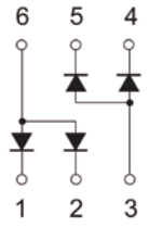
Equivalent Circuit
