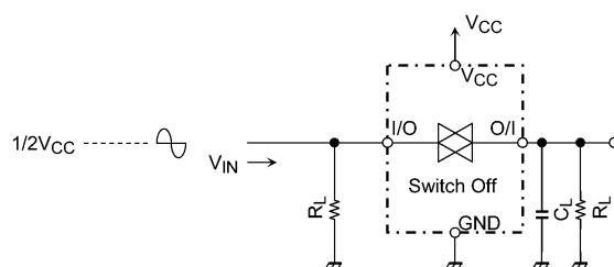
Figure 4 Feedthrough Attenuation
