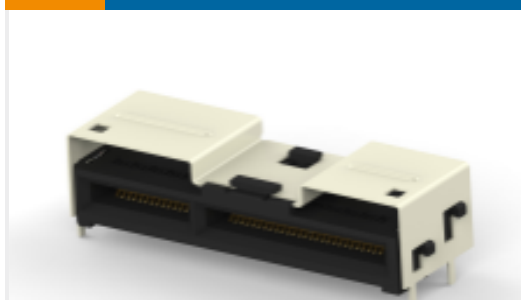
TE Part #2331814-1 CABLE REC ASSY, 84 P, RA, SLIVER 2.0
