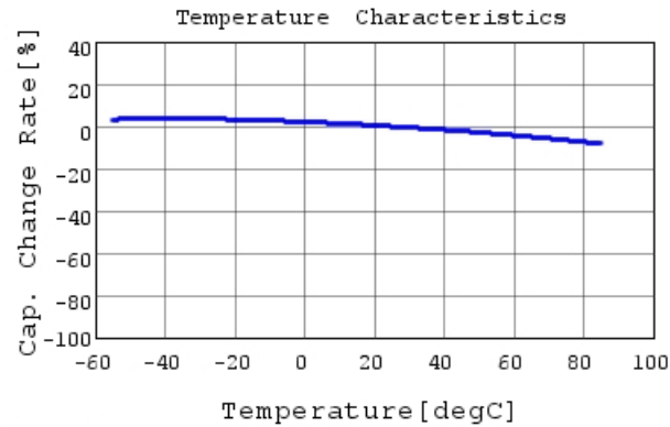
GRT033R61C103KE01 C-Temp. capchange, DC0.0V,
