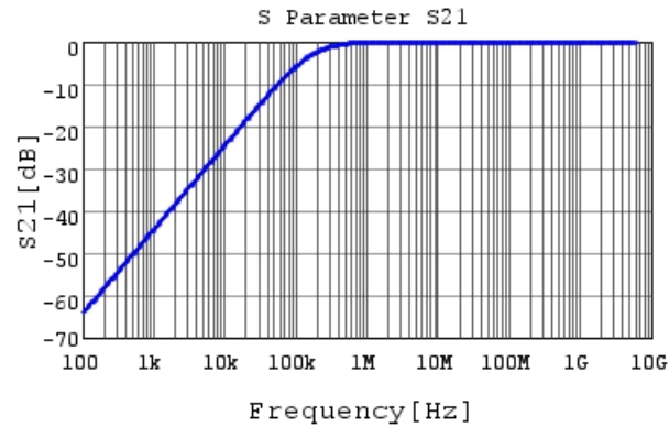
GRT033R61C103KE01 S21 DC0V, 25degC
